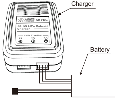
CONNECTION DIAGRAM
